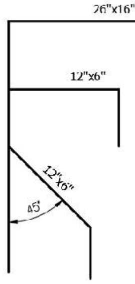
Mitered Elbows / Taps
